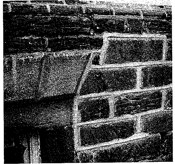
Figure 4. (left) The poor quality of this repointing—it appears to have been “tooled” with the mason’s finger—does not match the delicacy of the original beaded joint on this 19th-century brick wall. (right) It is obvious that the repointing on this “test patch” is not an appropriate replacement mortar joint for this early-19th century stone foundation. Photos: Lee H. Nelson, FAIA.
