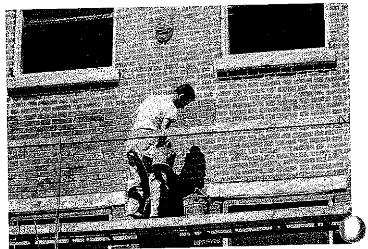
Figure 17. This photograph shows the significant visual change to the character of this historic brick building that has resulted from improper repointing procedures and a noticeably increased thickness of the mortar joints. Photo: Lee H. Nelson, FAIA.
