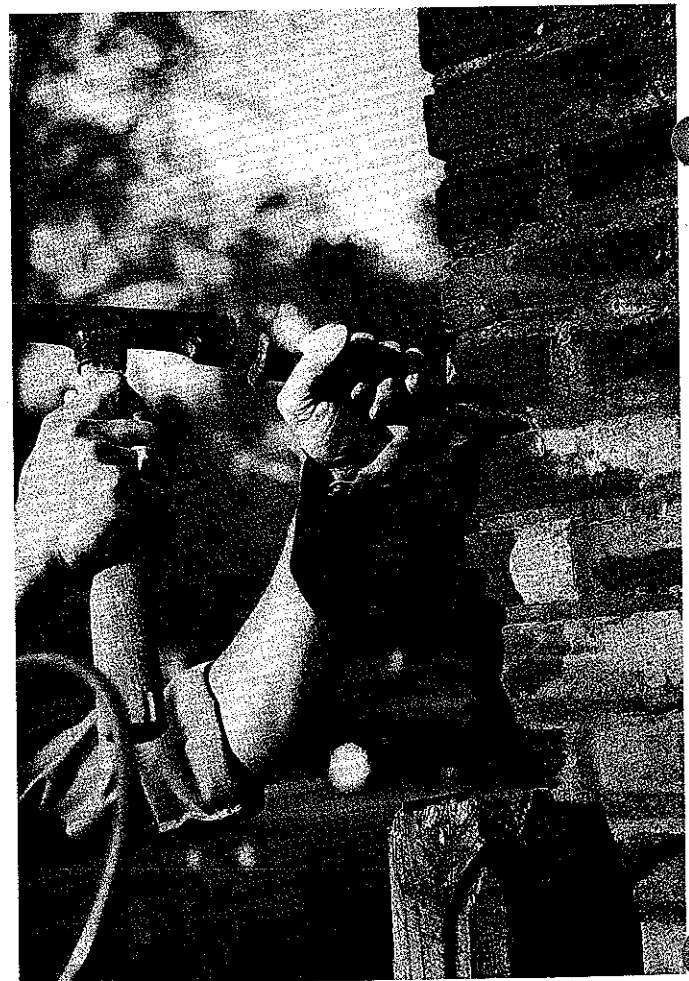
Figure 10. Using a hammer and masonry chisel is the least damaging and, thus, generally the preferred method of removing old mortar in preparation for repointing historic masonry. Photo: John P. Speweik.
